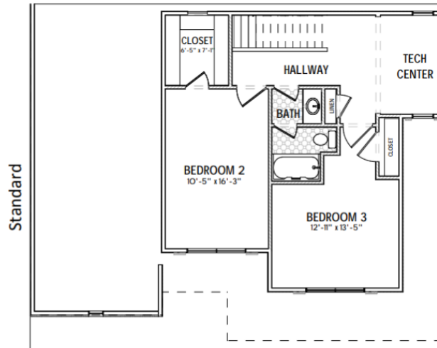
2nd Floor Plans
