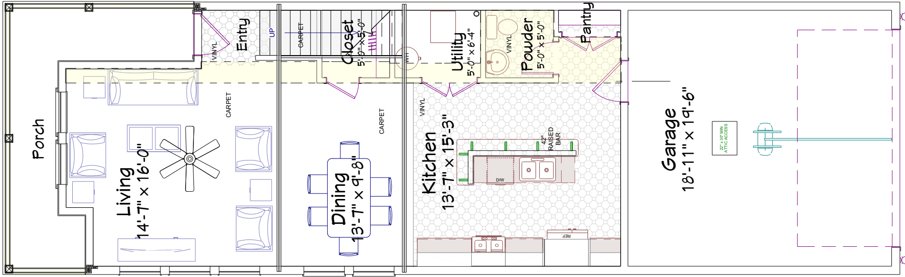
FIRST FLOOR LEVEL
