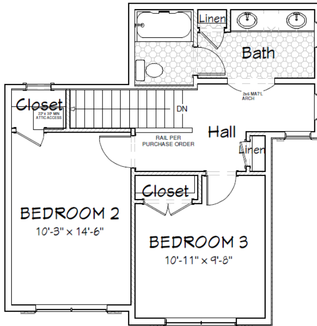
Standard Plan Upper Level
