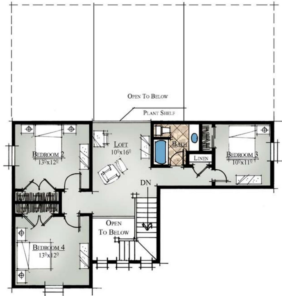
UPPER FLOOR PLAN 0' 4' 8' 1/8" = 1' - 0" ROOM DIMENSIONS ARE APPROXIMATE
